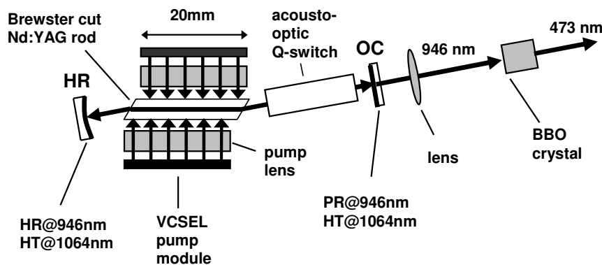
Figure 3: Schematic layout of the actively Q-switched VCSEL side-pumped Nd:YAG laser operating at the 946 nm transition. The laser output is frequency doubled in a non-linear BBO crystal.
